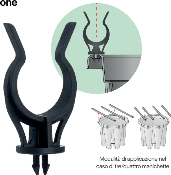
Application method for three/four hoses
