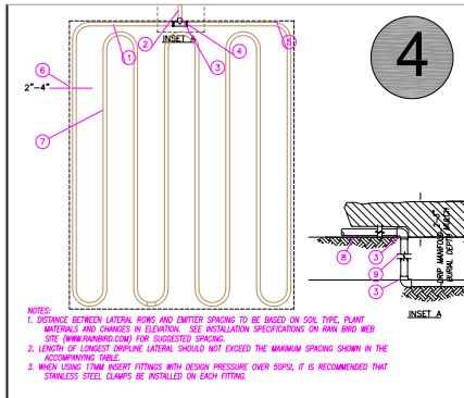
KFD ON-SURFACE DRIPLINE QUICK LAYOUT
