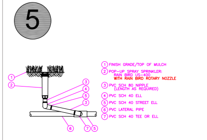
POP-UP SPRAY SPRINKLER QUICK LAYOUT
