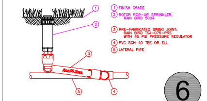
ROTOR POP-UP SPRINKLER QUICK LAYOUT
