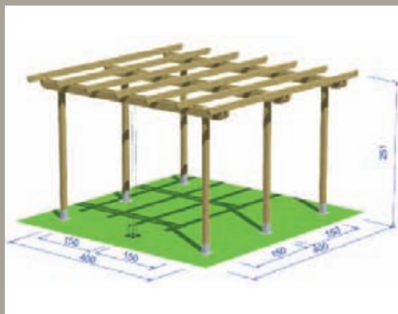
PERGOLA LUNA AUTOPORTANTE LUNA F.STAND. PERGOLA
