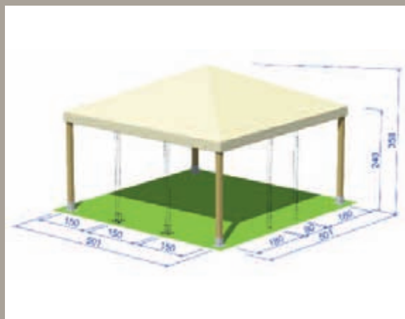
GAZEBO LE PIRAMIDI COPERTURA PVC LE PIRAMIDI GAZEBO, PVC COVERING
